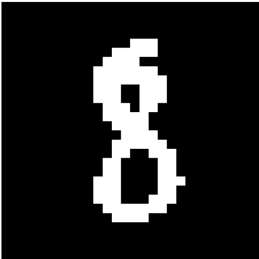
Original Input
