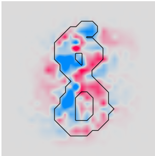
Feature Contribution
