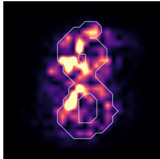
Absolute Importance
