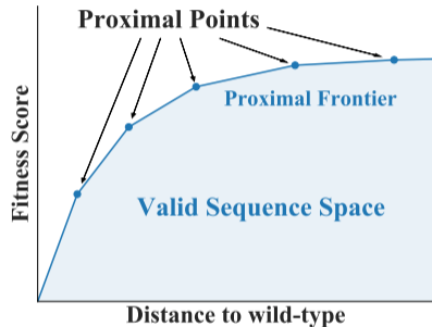
(a) Frontier of Proximal Points
